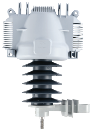
PDV-100 Optima Arrester with LA-13007 Wildlife Guard
