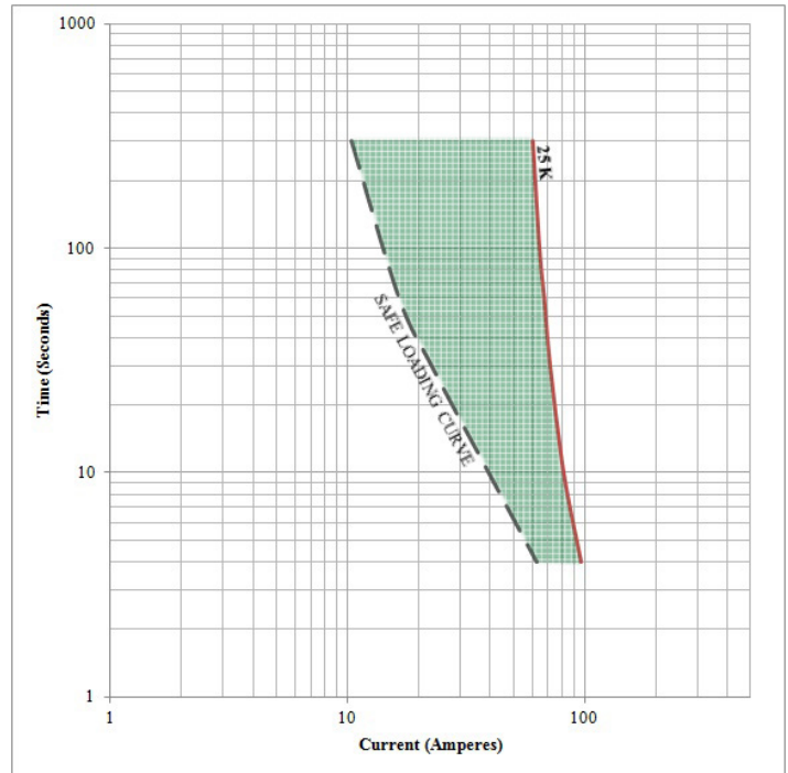
Figure 3 - Total Clearing Curve for NEMA 25 ampere “K” Fuse Link. Chance Catalog No. M25K23
