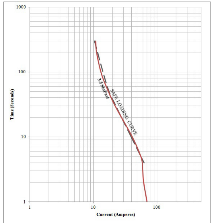
Figure 7 - Minimum melting time curve of Chance SloFast Fuse Link. Chance Catalog No. M3D5SF23.
