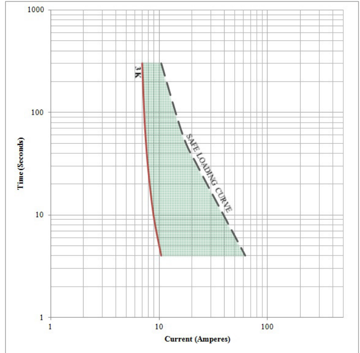
Figure 2 - Total Clearing Curve for NEMA 3 ampere “K” Fuse Link. Chance Catalog No. M3K23
