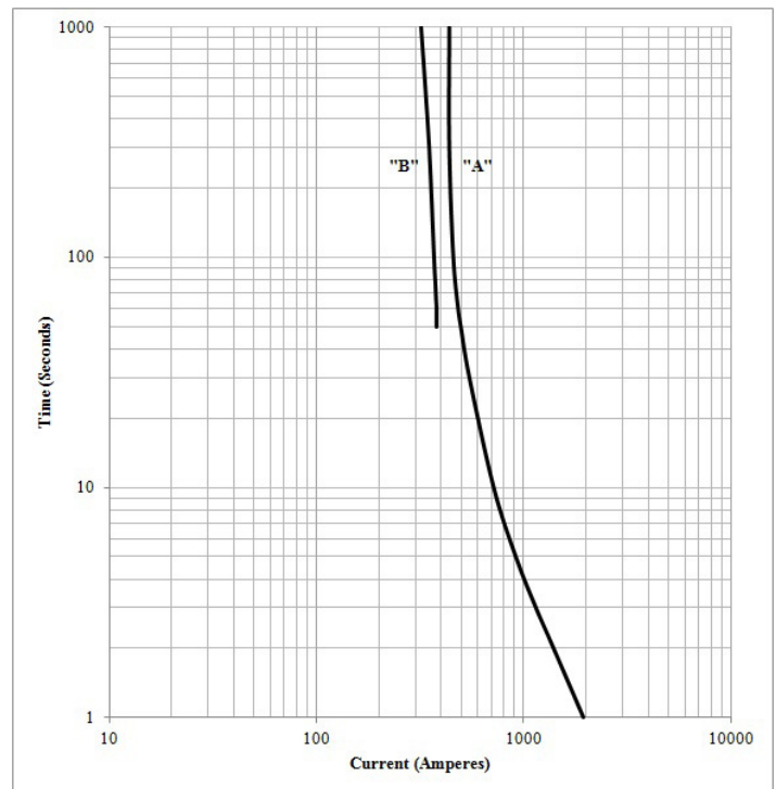
Figure 6 - Curve “A” 240V secondary breaker for 25 kVA, 7200V transformer. Curve derived from tests at 240V, 25°C ambient, no pre-loading. Curve “B” 240V secondary breaker for 25 kVA, 7200V transformer. Curve derived from tests, 70% pre-load, 35°C ambient, curve shown for 65°C transformer.
