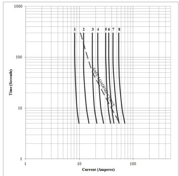
Figure 5 - Eight curves for fuses used as high-side internal fuses in self-protected transformers by one manufacturer. (The number designations are arbitrary and are not to be used as ampere ratings.)
