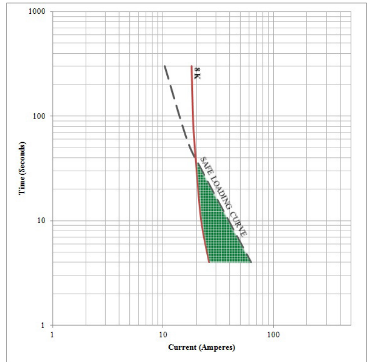
Figure 4 - Total Clearing Curve for NEMA 8 ampere "K" Fuse Link. Chance Catalog No. M8K23
