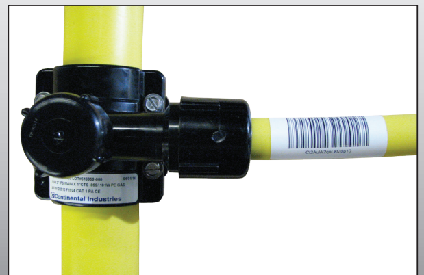
After installation, Bar Code Label may be placed on the Fitting, the Pipe or kept with your Paper Work
