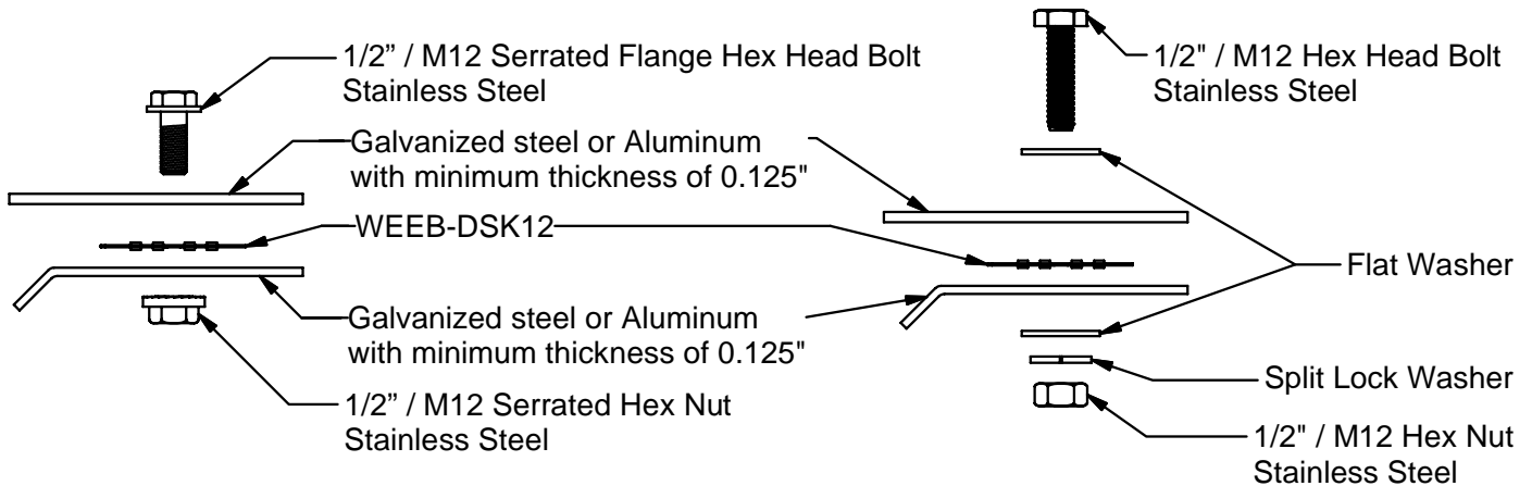
Fig 2: Mounting-With Washers
