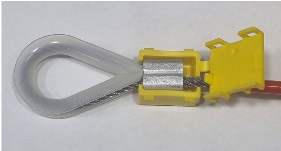
PHOTO 4: PROTECTIVE COVER SHOWN OPEN.
