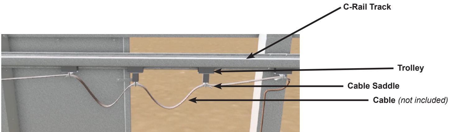
Tow Trolley Close-up
