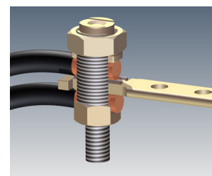
Traditional Split Bolt Option
