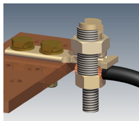
Terminating One Wire
