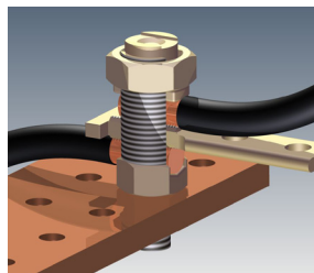
Two Wires to Busbar
