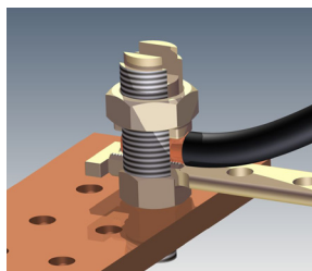
One Wire to Busbar
