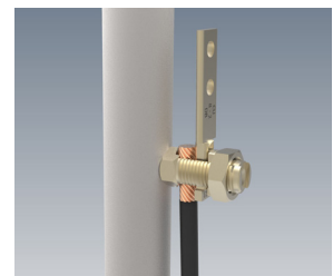
Wire to Pipe Connection
