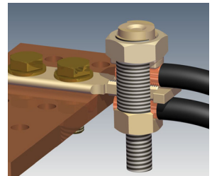
Terminating Two Wires
