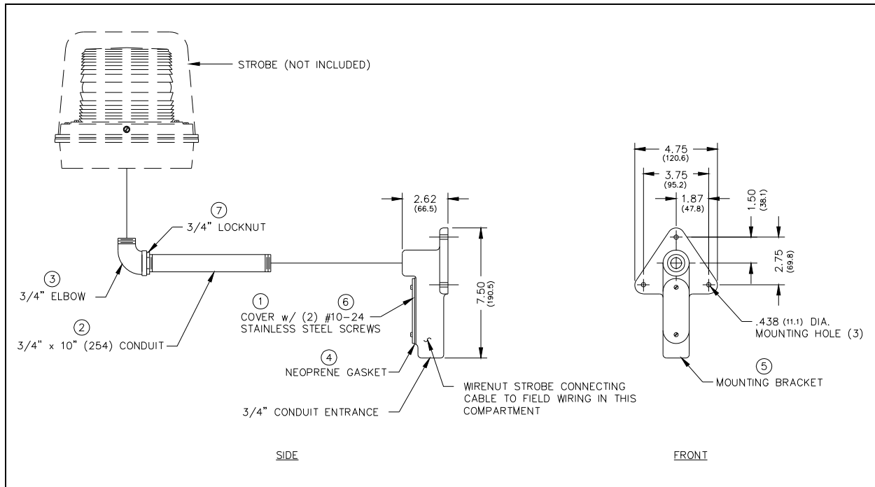
Figure 1. Strobe Mounting Details
