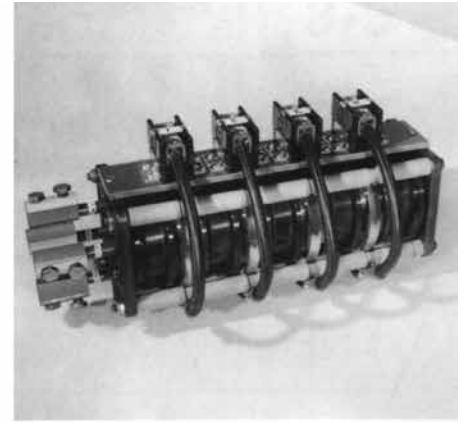
4-POLE, 200-AMP COLLECTOR
