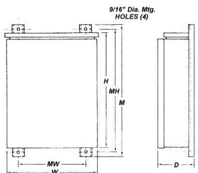
CABINET OUTLINE SIZE 1, 2, 3, 4 &amp; 5
