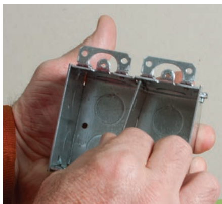
Step 3. Insert partition at slight angle then twist into position.
