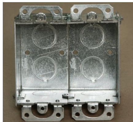
Step 2. Position boxes together leaving screws loose.
