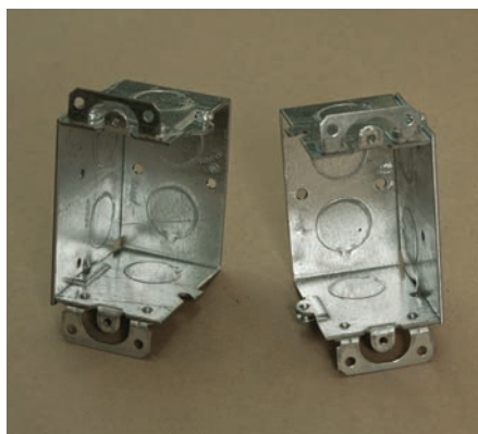
Step 1. Loosen screws and remove sides.
