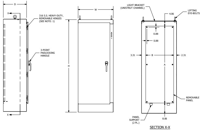
WRD72XM2718FS4
