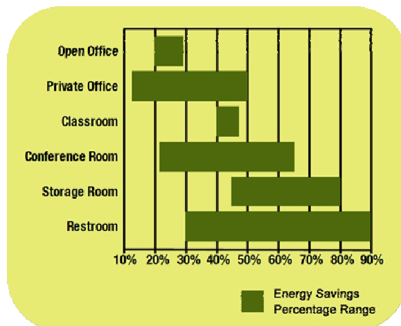
Potential Energy Savings Using Occupancy Sensors. Source: eSource
