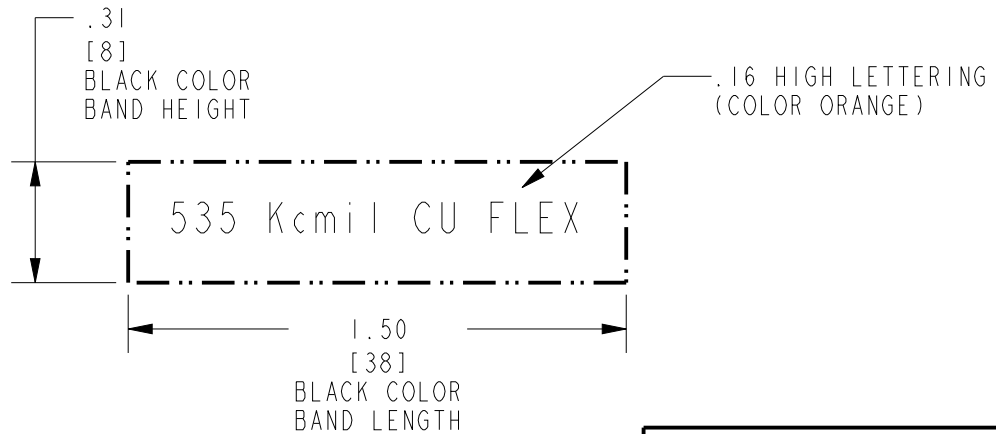
ENLARGED BAND VIEW (3 AROUND CIRCUMFERENCE)
