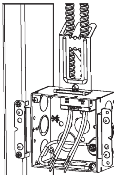
Step 5. Bend down two center tabs to lock cables as shown.
