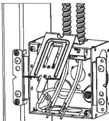
Step 3. Pre-bend Cable Support Bracket as shown and install cables.
