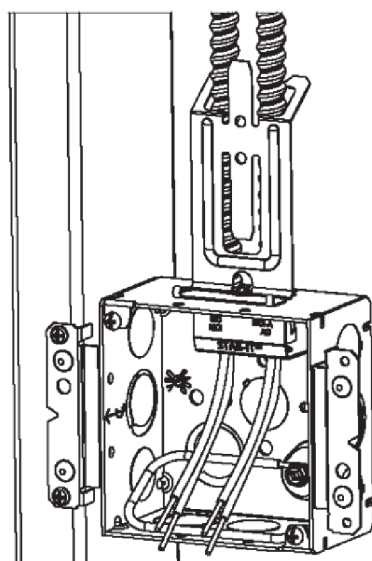
Step 4. Bend Cable Support Bracket as shown.
