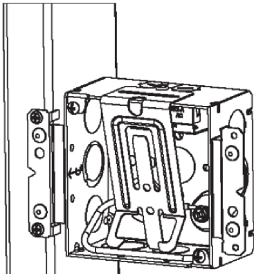
Step 1. Install box to stud.
