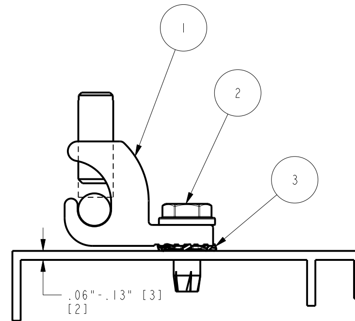
ANODIZED ALUMINUM INSTALLATION
