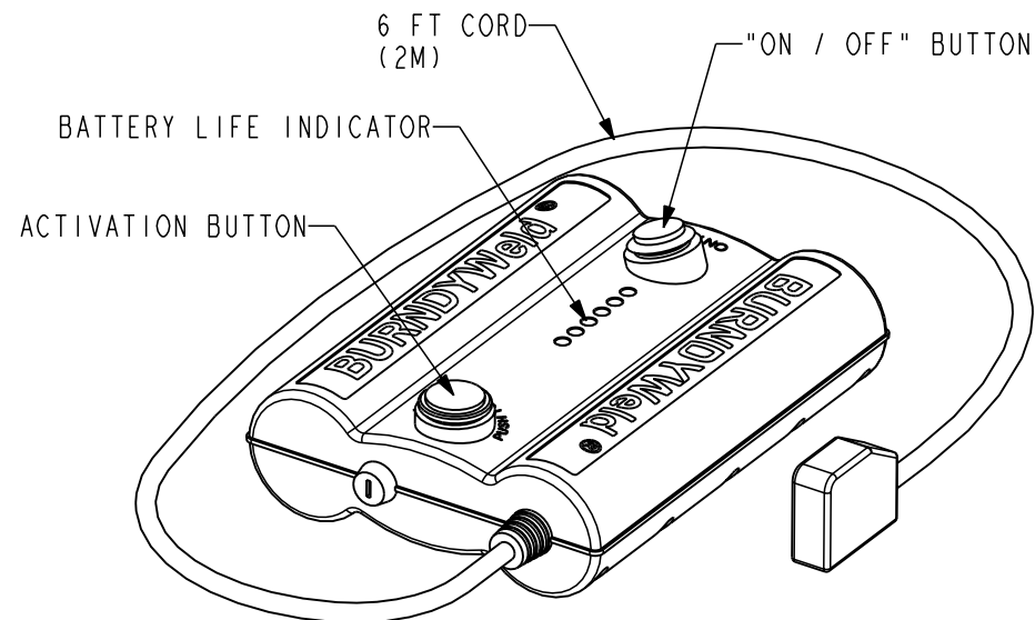
BURNDYWELD® QIKLITE™ IGNITION SYSTEM
