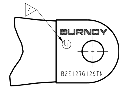
DETAIL A SCALE 3:2
