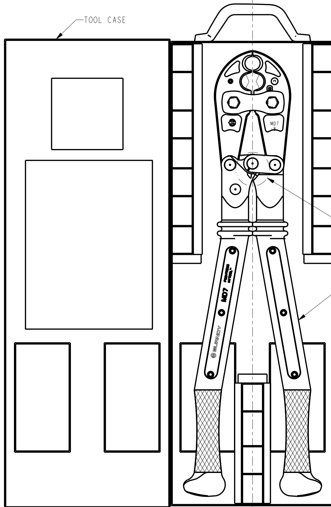
FIGURE 1 MD7-8 POSI-PRESS HYTOOL™
