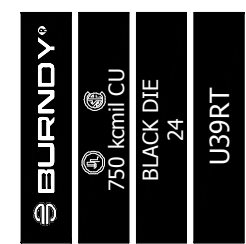
BARREL MARKING
