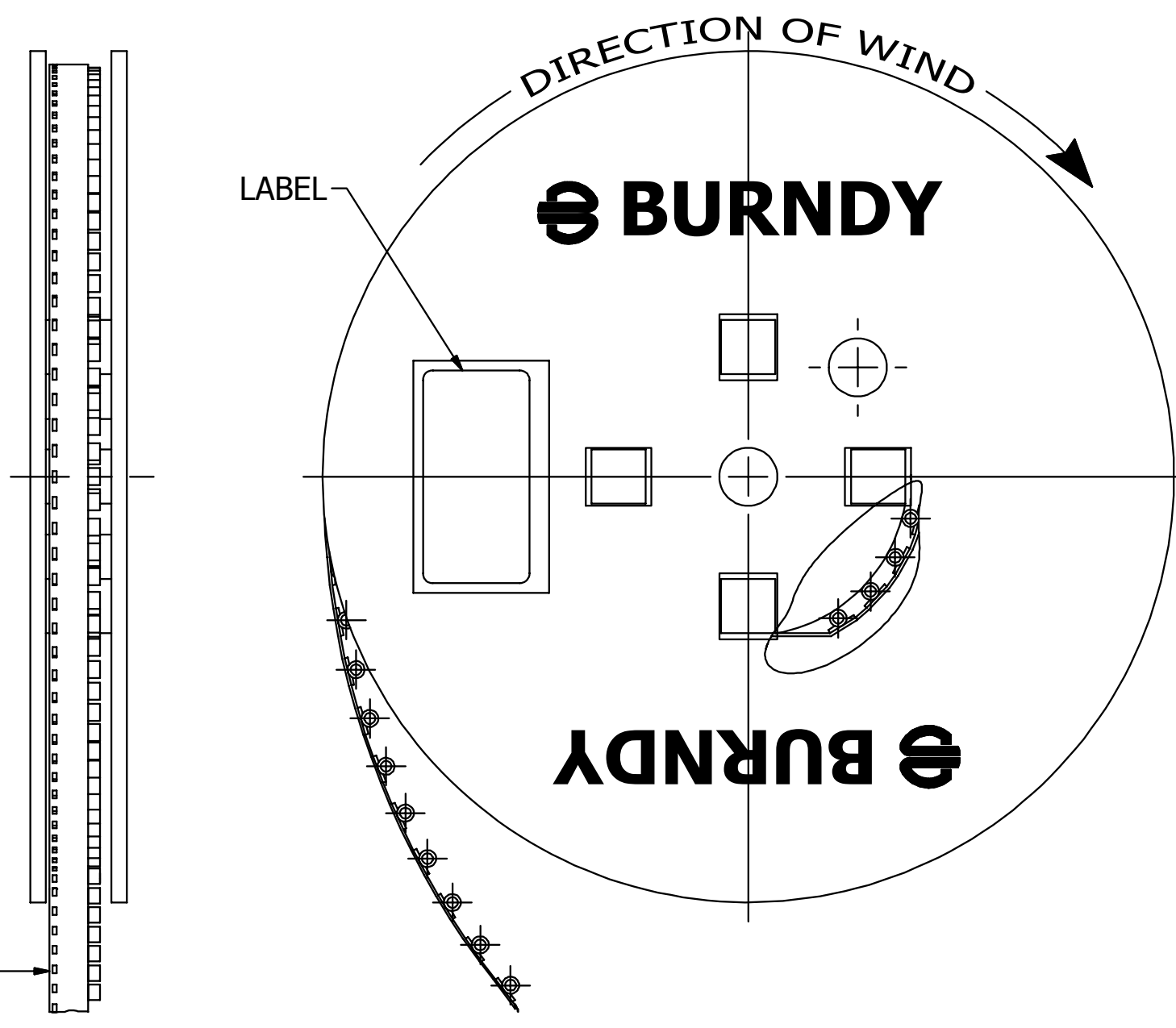
TYPICAL MYLAR STRIP WITH TERMINALS
