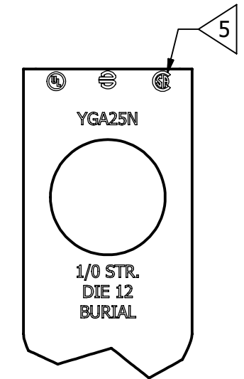
TYPICAL LETTERING
