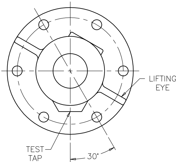
FLANGE ALIGNMENT DIAGRAM TOP VIEW
