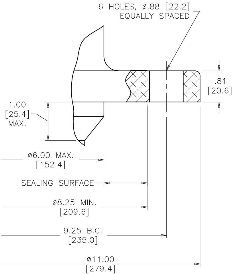
MOUNTING FLANGE DETAIL
