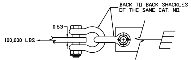
ULT. LOAD DIAGRAM
