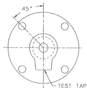
FLANGE ALIGNMENT DIAGRAM
