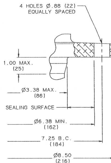
MOUNTING FLANGE DETAIL
