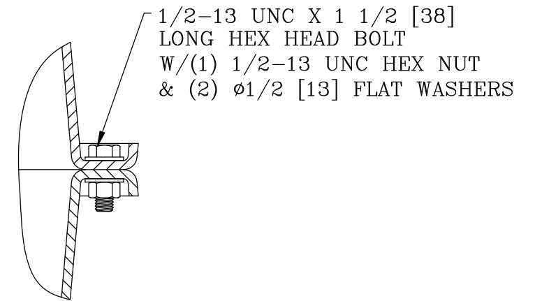
BOX ASSEMBLY DETAIL 3 PLACES
