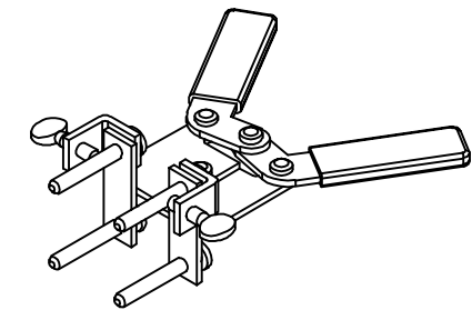
REF. 40-4565-00 HANDLE CLAMPS
