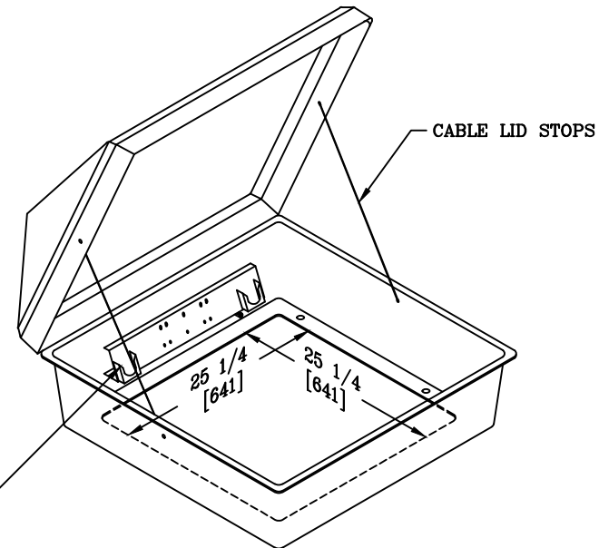
STAINLESS STEEL JUNCTION MOUNTING BAR W/COPPER GROUND LUG AND PARKING STANDS
