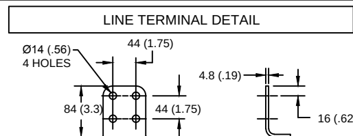
HDG 4-HOLE TERMINAL PAD, PART No. 274914-4002
