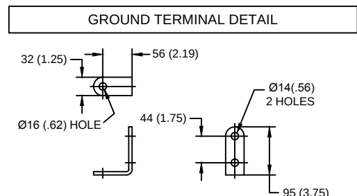
HDG 2-HOLE TERMINAL PAD, PART No. 271986-4002
