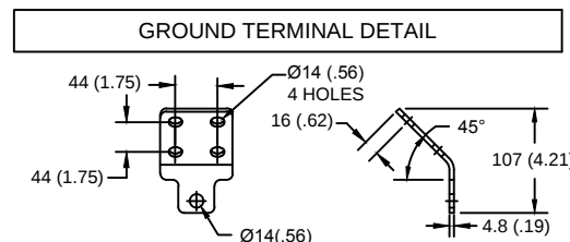
HDG 4-HOLE TERMINAL PAD, PART No. 274914-4001
