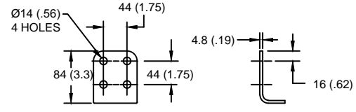
HDG 4-HOLE TERMINAL PAD, PART No. 274914-4002
