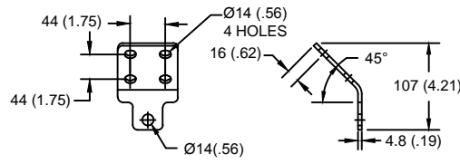
HDG 4-HOLE TERMINAL PAD, PART No. 274914-4001
