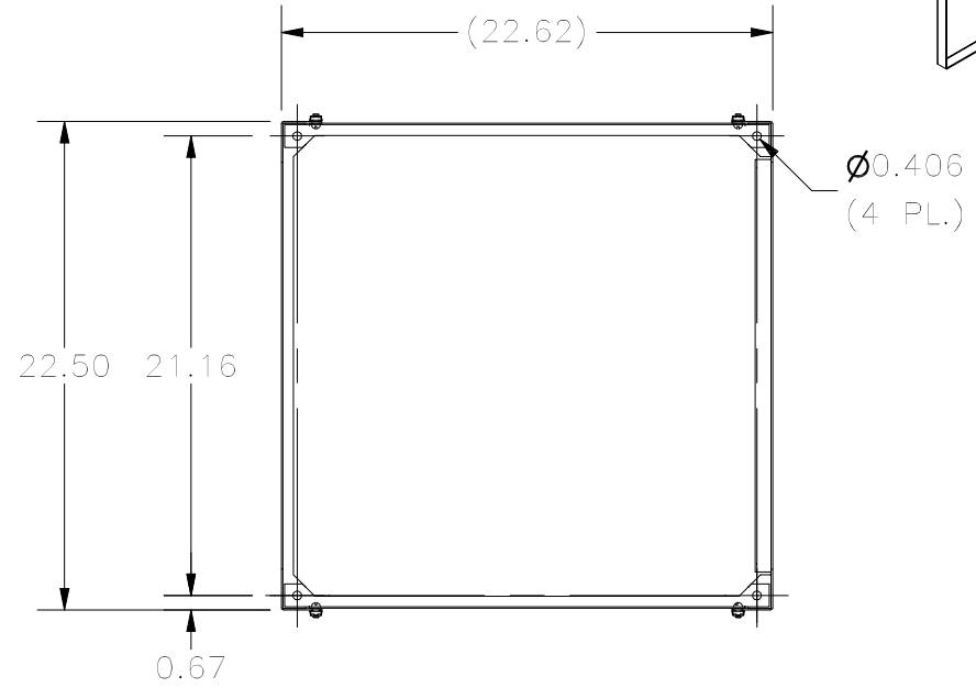
FRONT VIEW (SWING PANEL REMOVED)
