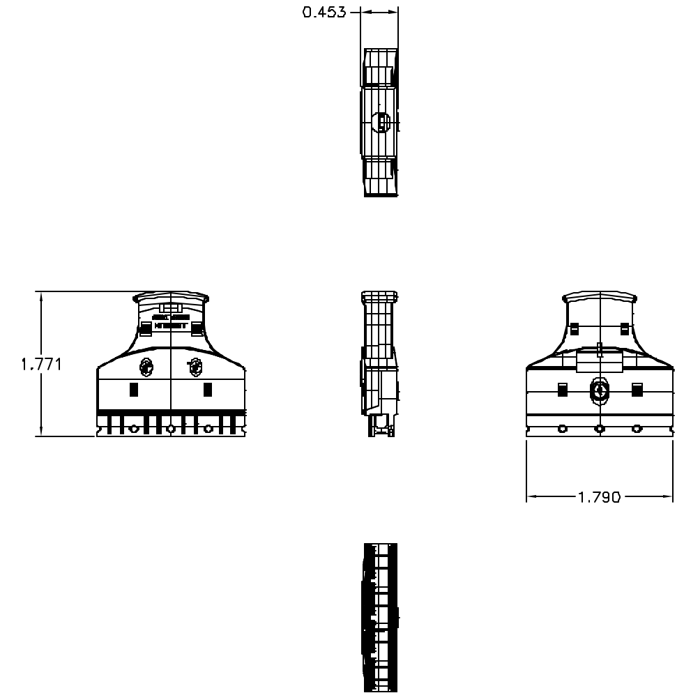
PLUG DETAIL
