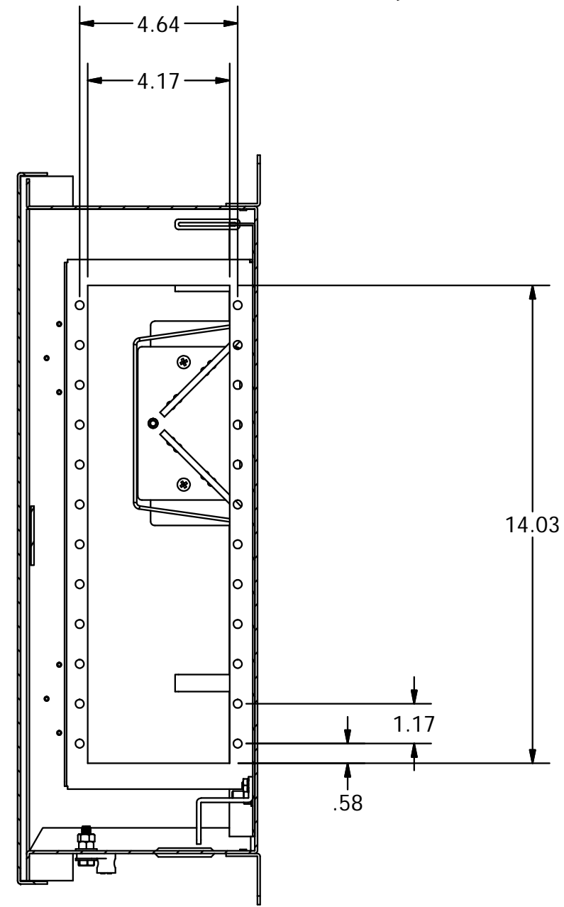
SECTION L-L SCALE 1 / 4
