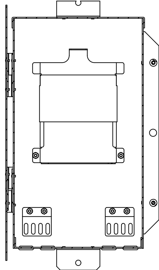
SECTION J-J SCALE 1 / 4
