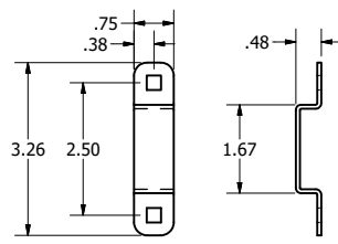
SUPPORT CLIP
