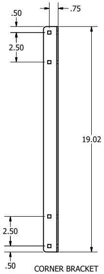
CORNER BRACKET
