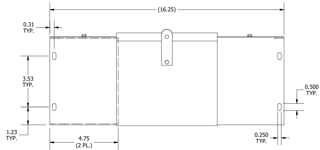
FRONT VIEW, FULLY EXTENDED VIEW
