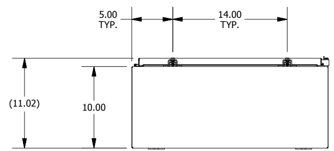
BOTTOM VIEW
