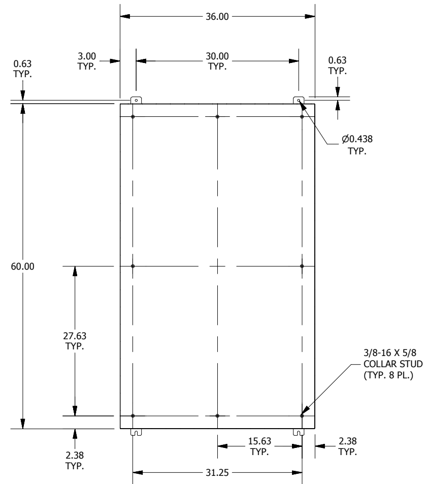
SECTION A-A (INSIDE BACK OF TUB)
