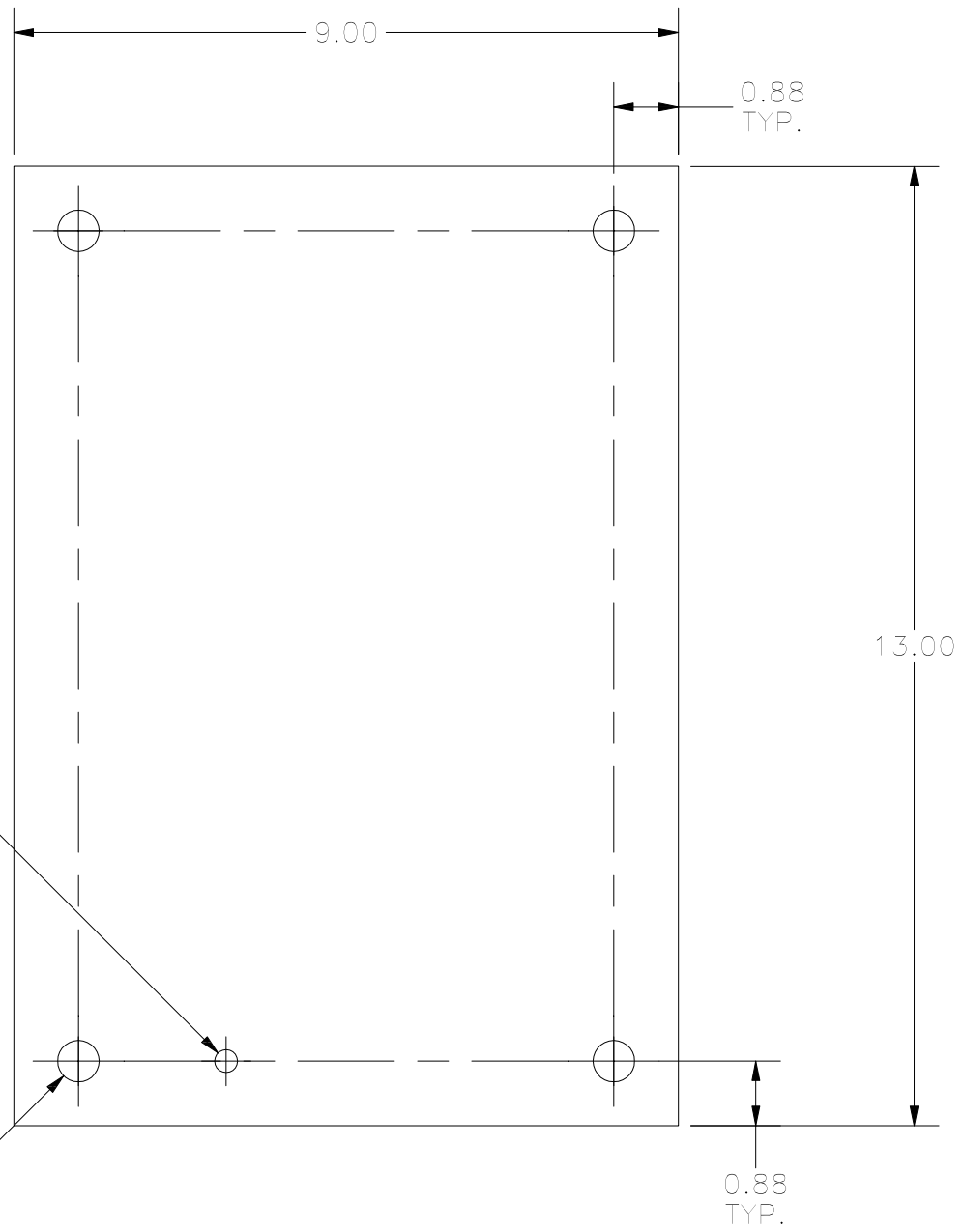
FRONT VIEW
