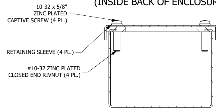
SECTION L-L VIEW (INSIDE TOP OF ENCL.)
