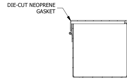
SECTION K-K (INSIDE BACK OF ENCLOSURE)
