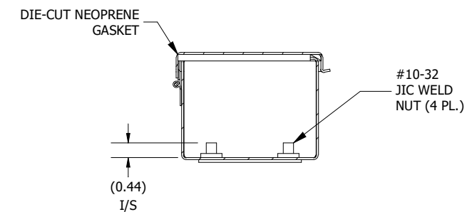
SECTION L-L VIEW (INSIDE TOP OF ENCL.)
