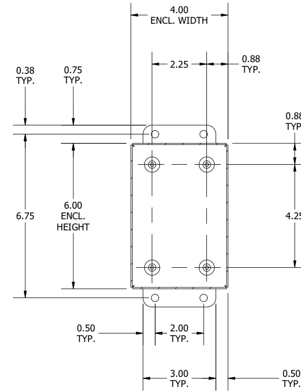
SECTION K-K (INSIDE BACK OF ENCLOSURE)
