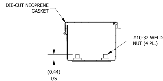
SECTION L-L VIEW (INSIDE TOP OF ENCL.)
