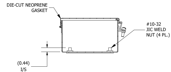
SECTION L-L VIEW (INSIDE TOP OF ENCL.)
