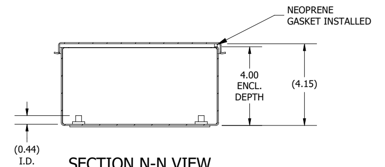
SECTION N-N VIEW (INSIDE TOP OF ENCL.)
