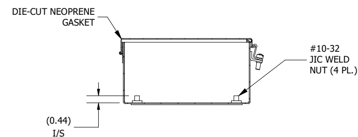
SECTION L-L VIEW (INSIDE TOP OF ENCL.)
