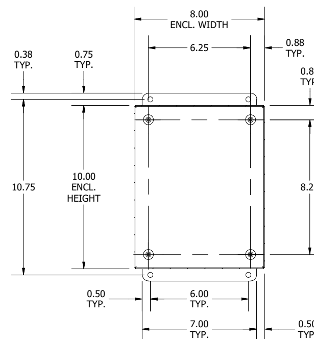
SECTION K-K (INSIDE BACK OF ENCLOSURE)
