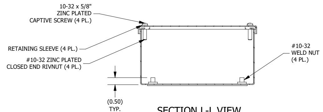
SECTION L-L VIEW (INSIDE TOP OF ENCL.)
