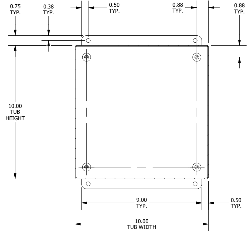
SECTION K-K (INSIDE BACK OF ENCLOSURE)
